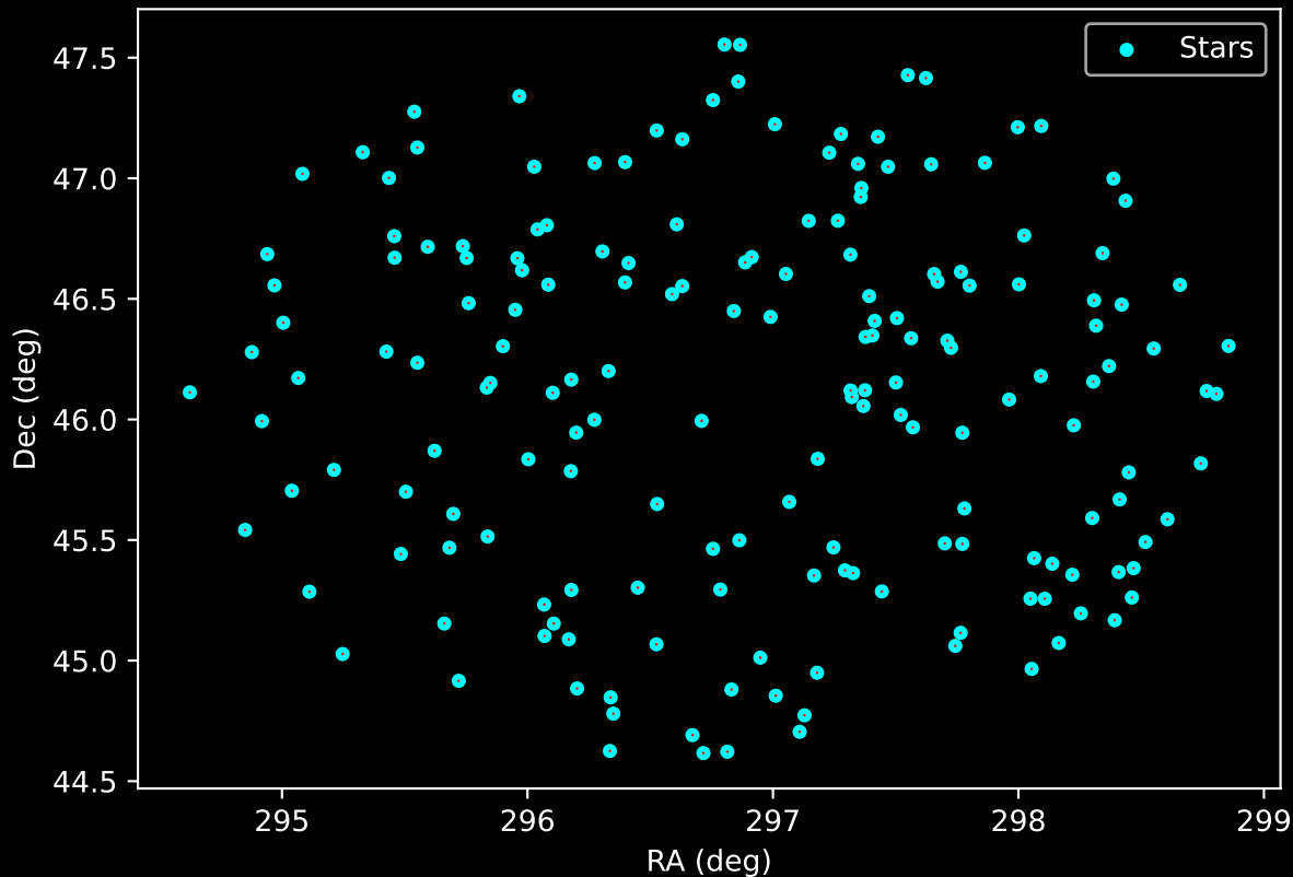
APOGEE DR17 Field: [115+71_MGA] Proper Motion Vectors for Gaia Star Field (n= 180)
