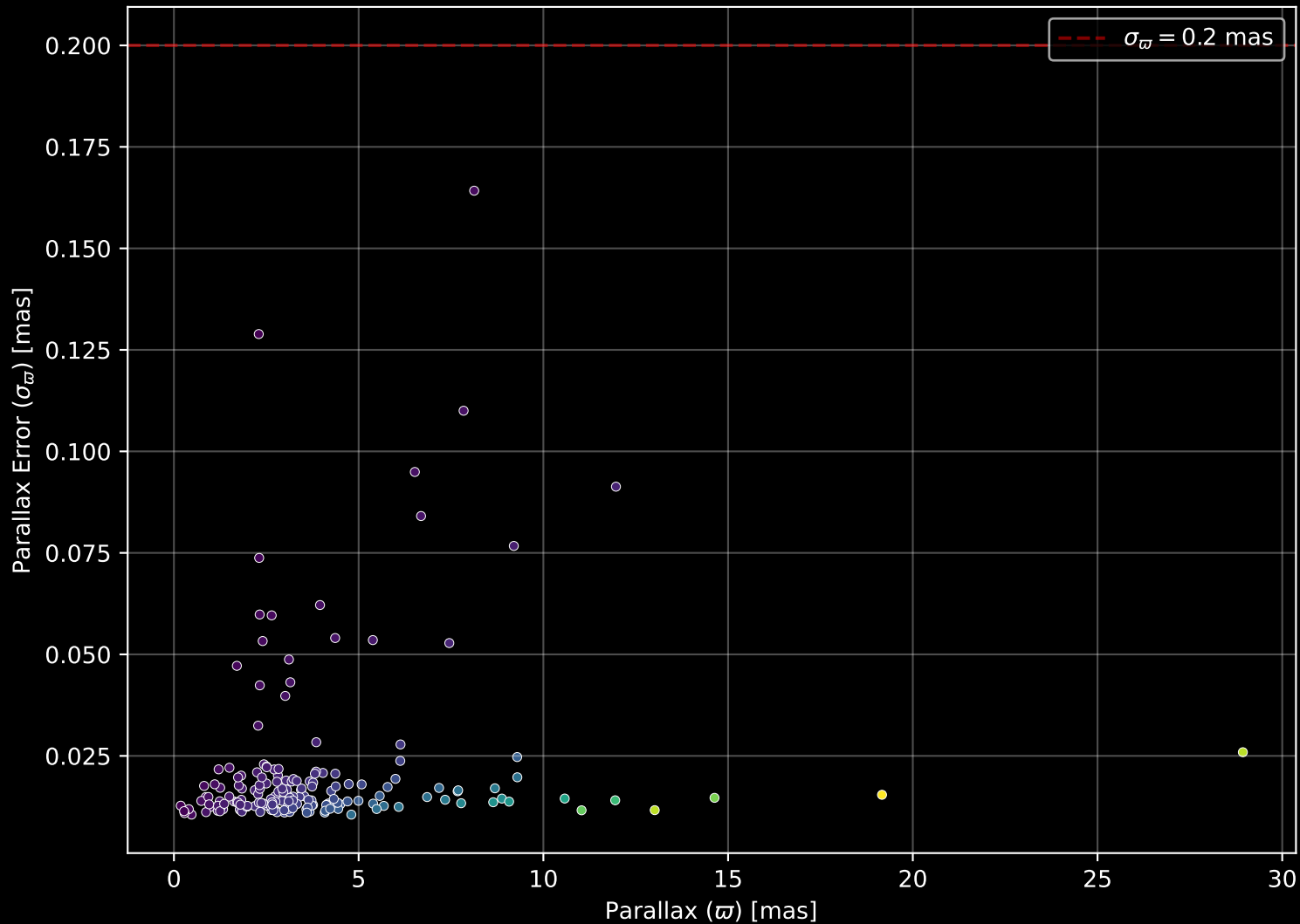
APOGEE DR17 Field: [115+71_MGA] Parallax Quality (n= 180)
