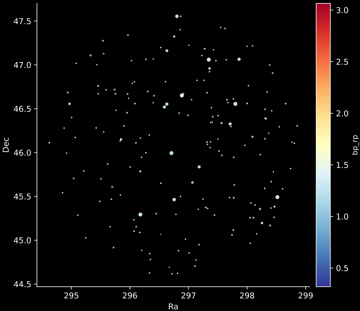
APOGEE DR17 Field: [115+71_MGA] Stars: 180
