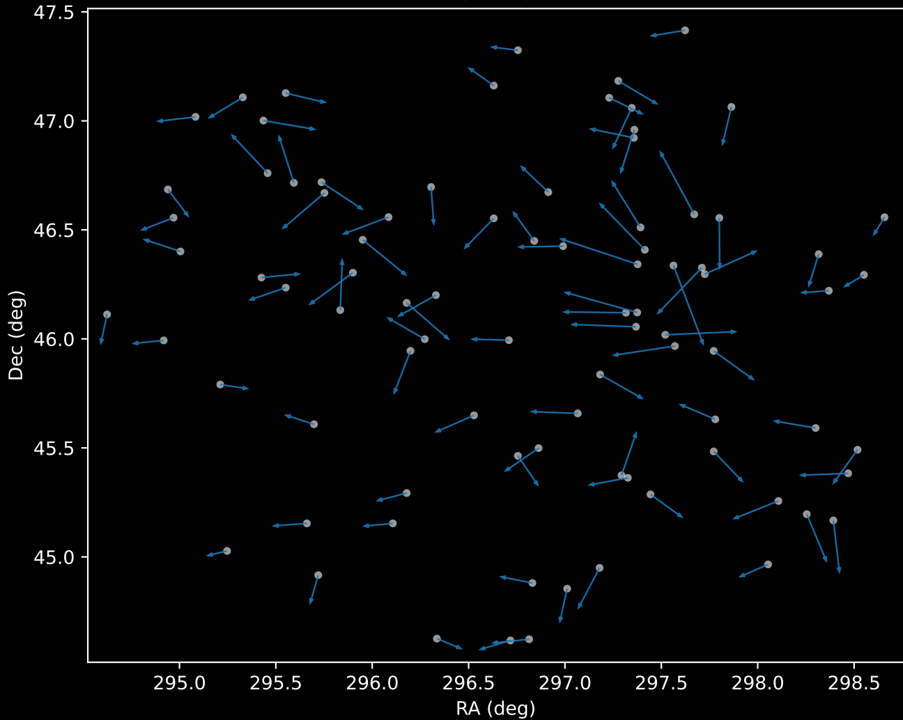
APOGEE DR17 Cluster 0 Proper Motion Vectors (n=86)
