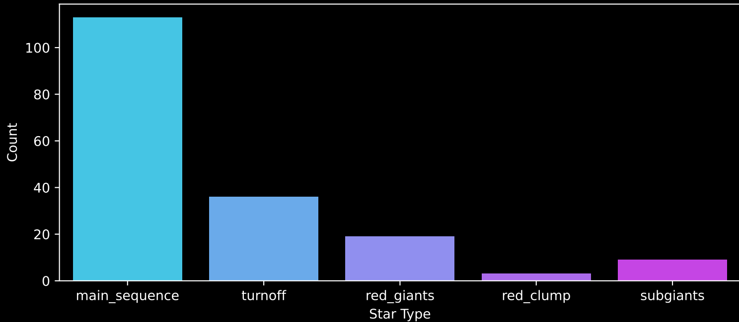
APOGEE DR17 Field: [115+71_MGA] Count plot of Star Type
