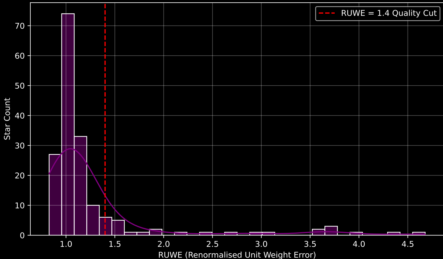
GAPOGEE DR17 Field [115+71_MGA] RUWE Distribution (n= 172)
