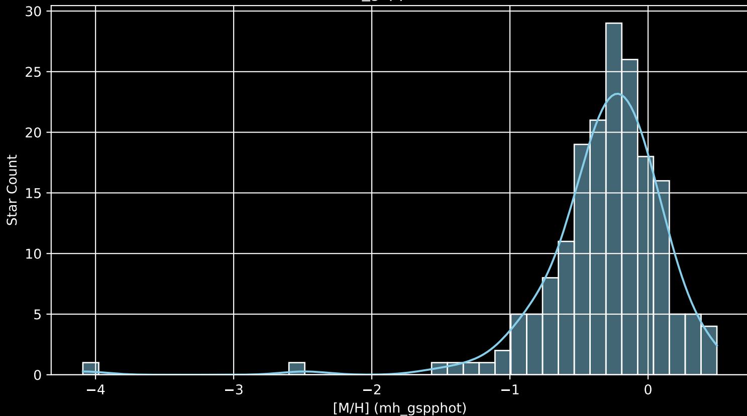
APOGEE DR17 Field: [115+71_MGA [M/H] (mh_gspphot) (n= 180)
