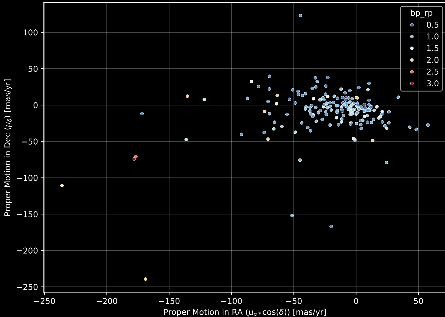
APOGEE DR17 Field: [115+71_MGA] Proper Motion Diagram (n= 180)
